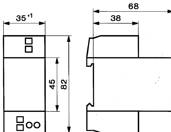
Taxxo 403 – dimensional details
